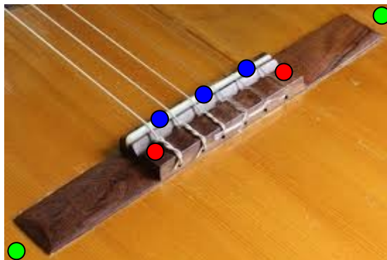
Fig. 5. Arrangement for structural and radiation measurements on guitars, with locations of introducing mechanical impulses with a light hammer (blue), locations of acceleration measurement (red) and locations of sound pressure measurement 10 cm above green marks.
