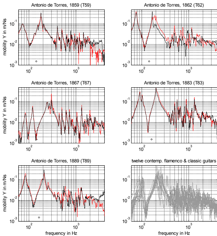
Fig. 7. Mobility plots of Torres guitars T59, T62, T67, T83, T89, and of twelve contemporary classic and flamenco guitars. Mobility measured according to Fig. 5 on the treble side (red) and the bass side (black) of the bridge. Resonance of the Helmholtz cabinet f_0 as determined by volume alone is indicated by black circles.
