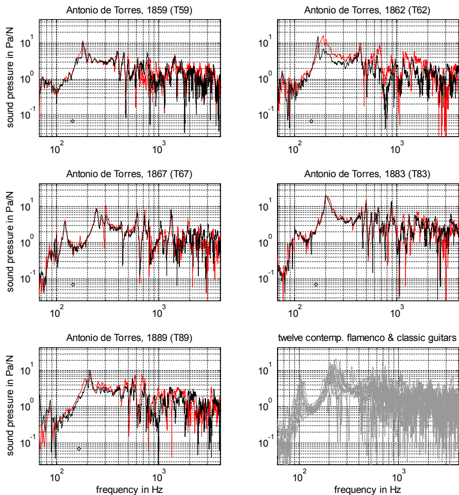
Fig. 10. Radiation plots of Torres guitars T59, T62, T67, T83, T89, and of twelve contemporary classic and flamenco guitars. Radiation measured according to Fig. 5 on the treble side (red) and the bass side (black) of the bridge. Resonance of the Helmholtz cabinet f_0 as determined by volume alone is indicated by black circles.
