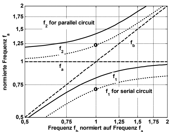
Fig. 4. Normalized frequencies f_1 and f_2 resulting from coupling two system components with individual stand-alone frequencies f_a and f_b , when coupled by a factor of k = 0.5 .
