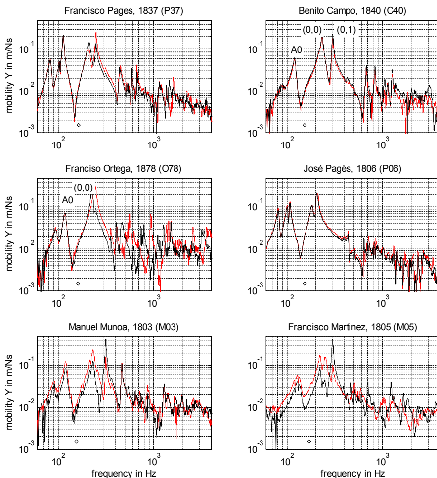
Fig. 6. Mobility plots of romantic guitars P37, C40, O78, P06, and the early romantic guitars M03 and M05. Mobility measured according to Fig. 5 on the treble side (red) and the bass side (black) of the bridge. Resonance of the Helmholtz cabinet f_0 as determined by volume alone is indicated by black circles.
