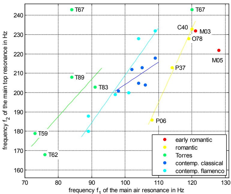
Fig 8. Frequency of the main top resonance, the (0,0) mode when coupled to the air cabinet in the assembled guitar versus the frequency of the main air resonance, for various epochs of guitar making. For acronyms see Table 1, for non-labelled examples of guitars see text.
