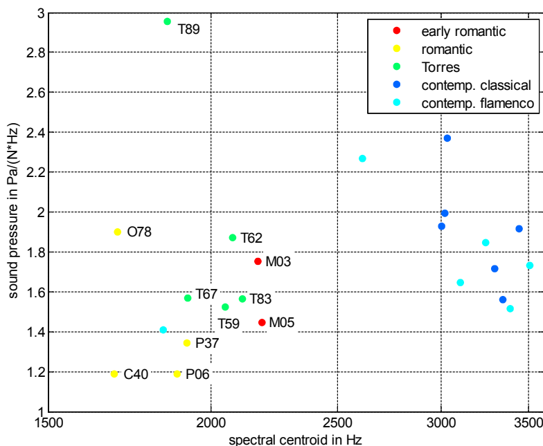
Fig. 12. Sound pressure normalized to impact force and to bandwidth in the range of 50 Hz to 4000 Hz versus spectral centroid at a sample rate of 12 kHz for guitars of various epochs. For acronyms see Table 1, for non-labelled examples of guitars see text.
