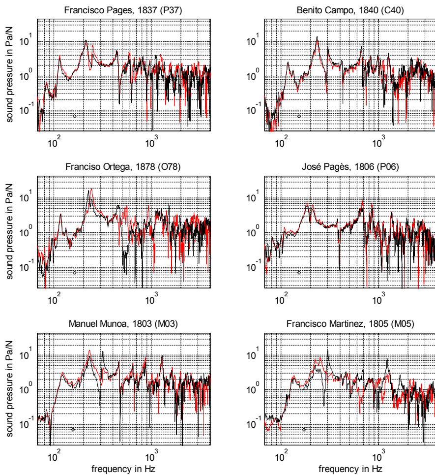
Fig. 9. Radiation plots of romantic guitars P37, C40, O78, P06, and early romantic guitars M03 and M05. Radiation measured according to Fig. 5 on the treble side (red) and the bass side (black) of the bridge. Resonance of the Helmholtz cabinet f_0 as determined by volume alone is indicated by black circles.
